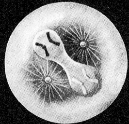
(4) NUCLEI FUSE
